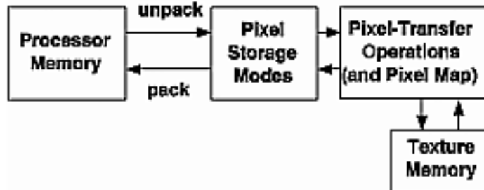
Figure 8-7 glTexImage*() , glTexSubImage*() , and glGetTexImage() Pixel Paths
