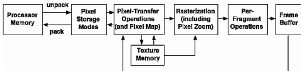
Figure 8-4 Imaging Pipeline
