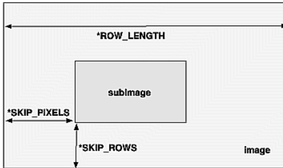
Figure 8–9 *SKIP_ROWS, *SKIP_PIXELS, and *ROW_LENGTH Parameters
