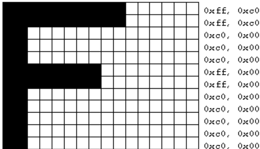
Figure 8-1 Bitmapped F and Its Data
