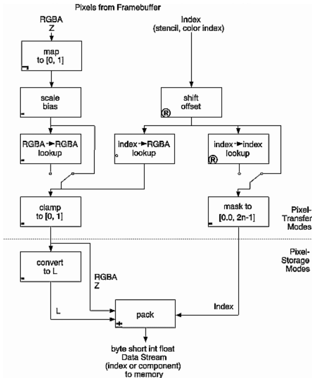
Figure 8–11 Reading Pixels with glReadPixels()
