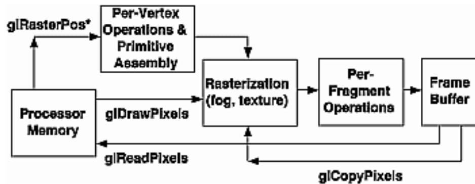
Figure 8-3 Simplistic Diagram of Pixel Data Flow
