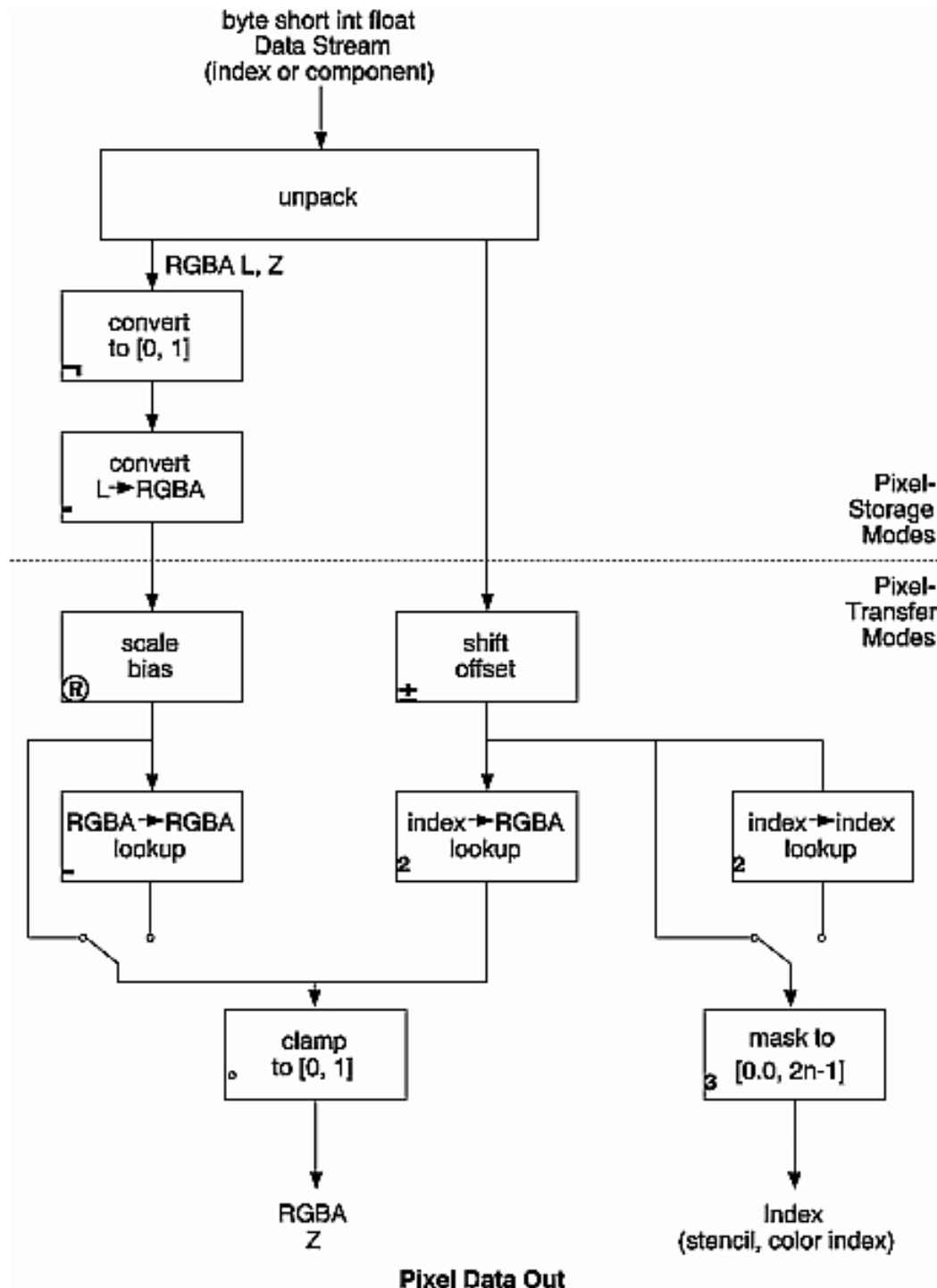
Figure 8–10 Drawing Pixels with glDrawPixels()
