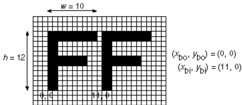
Figure 8–2 Bitmap and Its Associated Parameters
